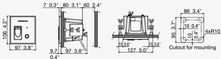
Multi Function Display Black Box TZT2BB Switch Box PSD-003 0.75 kg 1.7 lb
